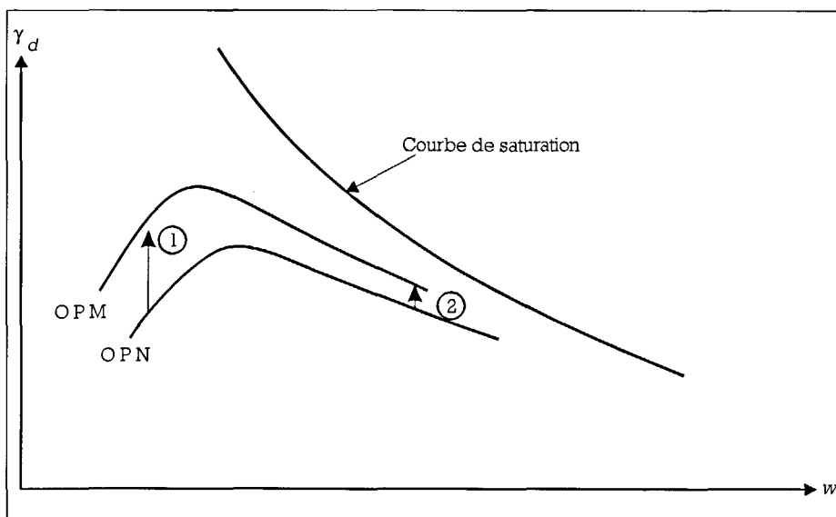
Figure 4 - Courbes Proctor.
